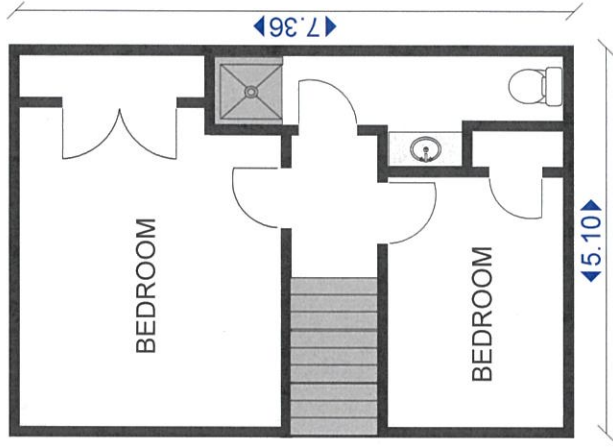
Grey 2 Storey - Top floor 38m 2 Scale 1:100
